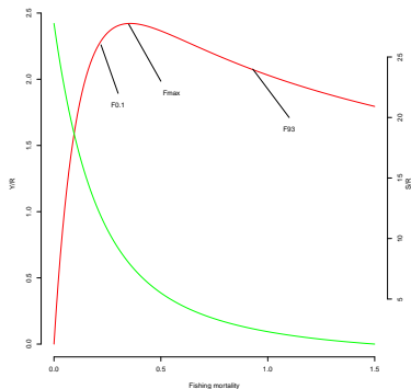
Figure : F over F_{0.1} gives little extra yield but much less SSB.
