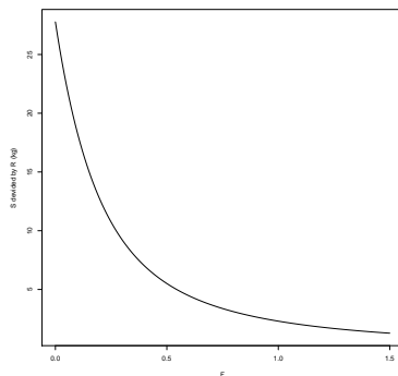
Figure : Spawning stock biomass per recruit for a simulated stock
