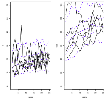
Figure : Example of medium-term prediction of SSB trend with uncertainty in initial stock size, recruitment, and annual assessment.
